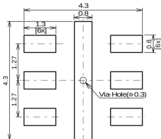
Fig.4 Desirable land area (in mm)
