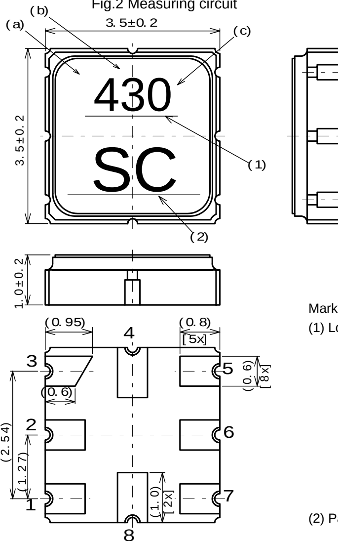
Fig.3 Package dimensions (in mm)
